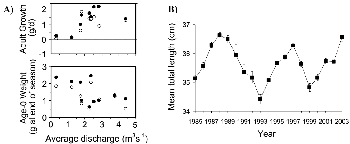
Figure 2-6 A) Adult and young-of-the-year (YOY) grayling growth versus mean summer river discharge in the Kuparuk River. Adult fish growth is higher when discharge is high, whereas YOY grow best during low flow summers. B) Mean total length ( \pm SE) of Kuparuk River grayling over time. Changes in mean length reflect the recruitment resulting from favorable years for YOY growth and survival.
