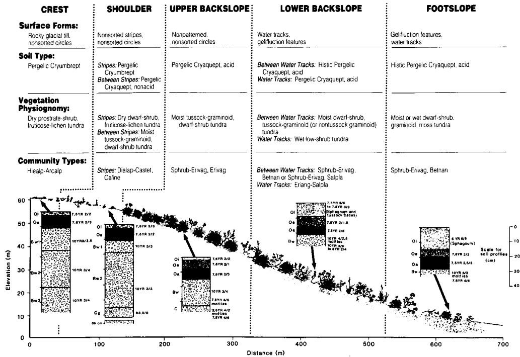
Figure 2-4. A typical toposequence of Sagavanirktok age (~300,000 y), in the Imnavait Creek drainage (Walker et al. 1989). This is one of the toposequences to be studied intensively by the Terrestrial and Landscapes Interactions groups, focusing on downslope water and element movement. It is underlain by permafrost at a depth of 30-150 cm
