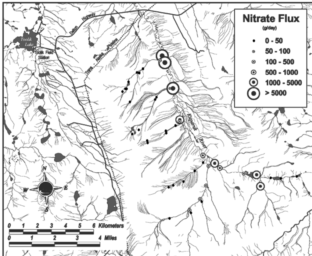
Figure 2-7. Synoptic sampling of streams in the Upper Kuparuk watershed was conducted for discharge and water chemistry on July 6, 2003. Figure shows the distribution of nitrate flux throughout the stream network. Most tributaries show low nitrate export but there are both source and sink hotspots that dominate nitrate dynamics in the watershed.
